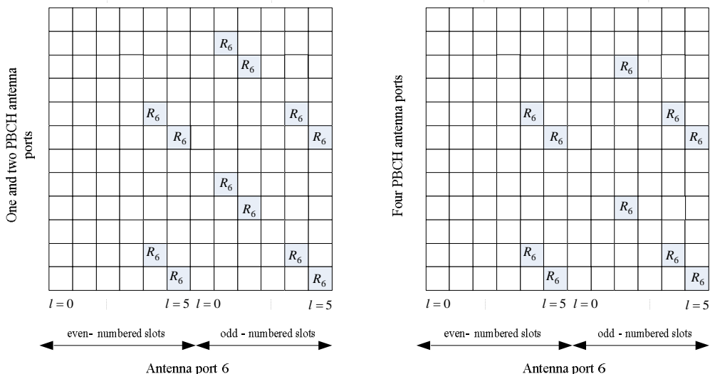
Figure 6.10.4.2-2: Mapping of positioning reference signals (extended cyclic prefix)
